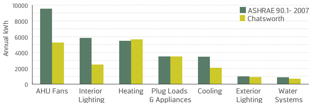
Figure 2. Overall efficiency savings are driven by reductions in air handler fans, interior and exterior lighting and domestic hot water.
