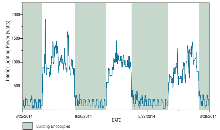
Figure 4. Total interior lighting power with spikes highlighted during several evenings when the building is unoccupied.
