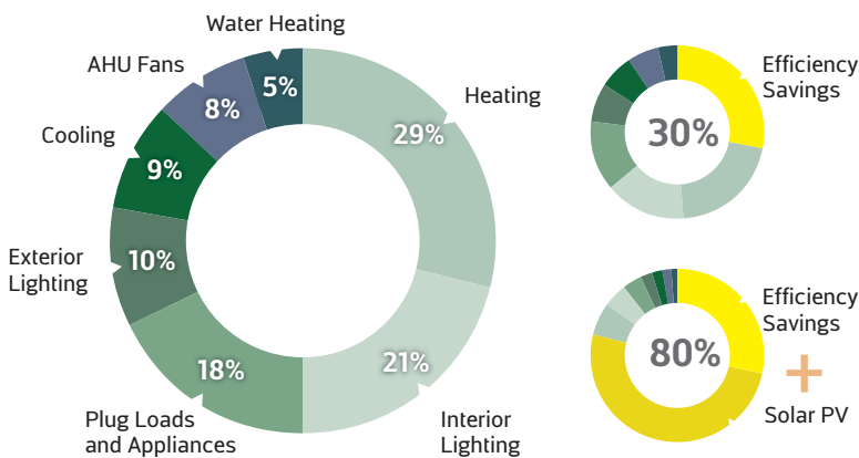
Figure 2. Overall efficiency savings are driven by reductions in interior lighting, cooling, air handler fans, heating, and exterior lighting energy use.
