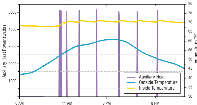
Figure 3. Auxillary heat power consumption compared to outside temperature. Strip heat power consumption (purple line) on a day when outside temperatures (blue line) never fell below 42°F.
